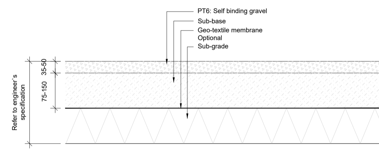
6 PT6: Self binding gravel scale 1:10 @A1
