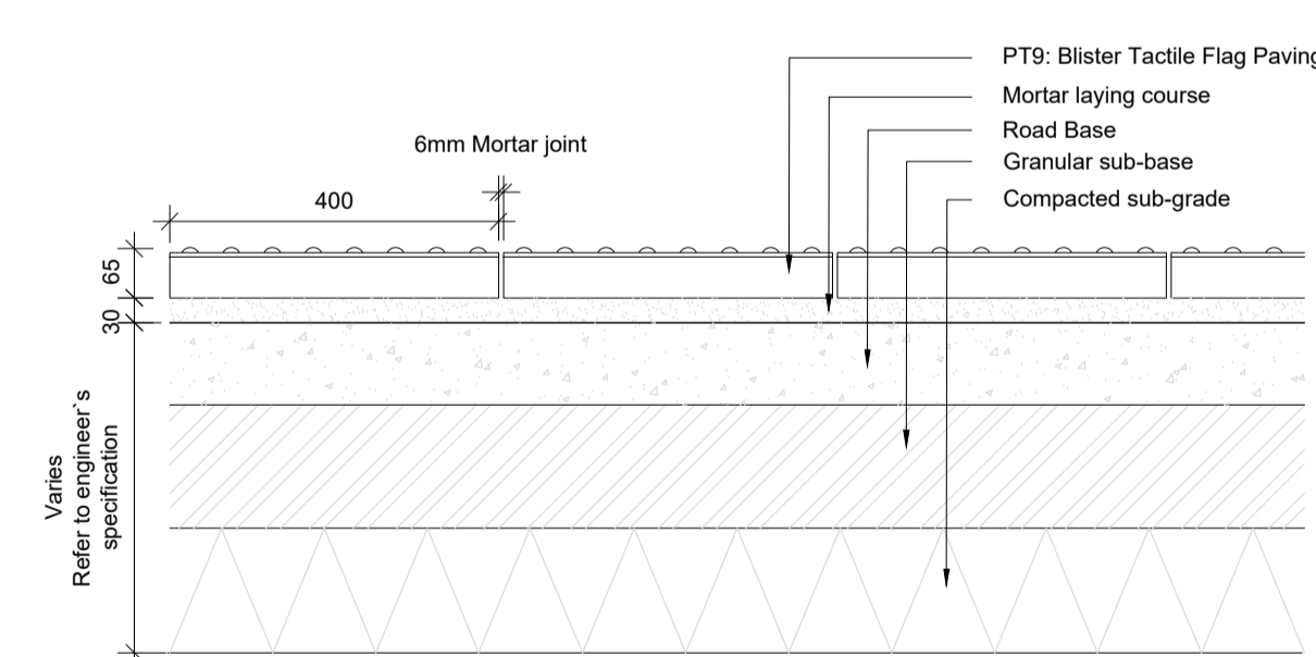
8 PT9: Blister tactile flag paving scale 1:10 @A1
