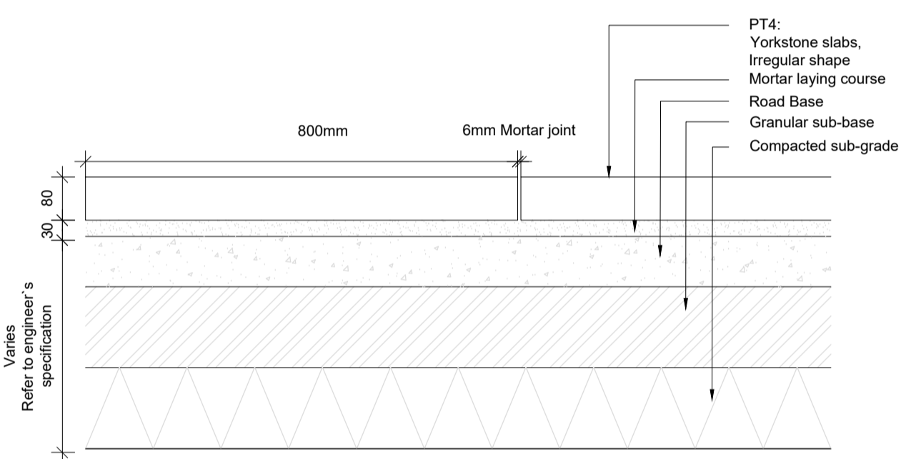
4 PT4: Yorkstone slabs, Irregular shape scale 1:10 @A1
