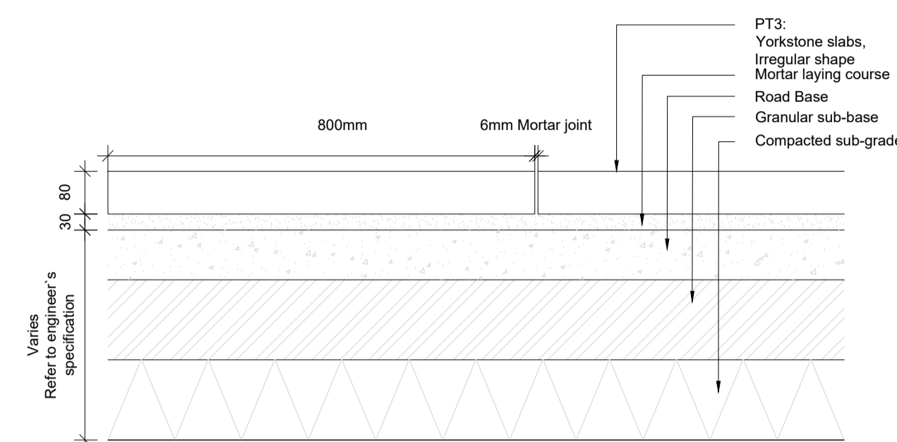
3 PT3: Yorkstone slabs, Irregular shape scale 1:10 @A1
