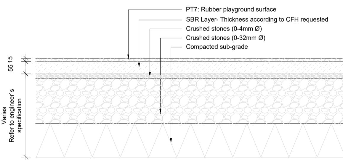
7 PT7: Rubber playground surface scale 1:10 @A1
