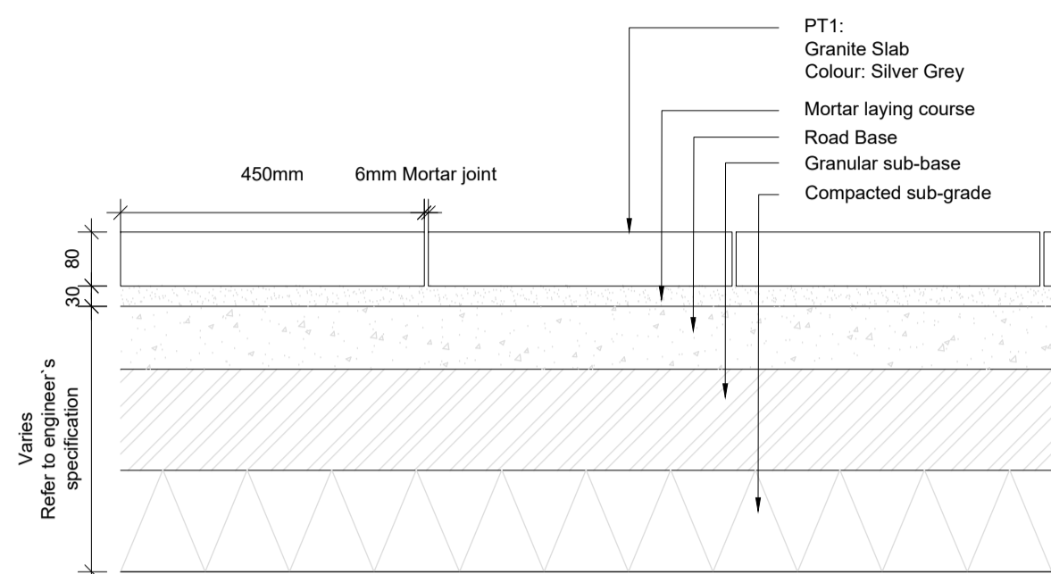
1 PT1: Granite slabs scale 1:10 @A1
