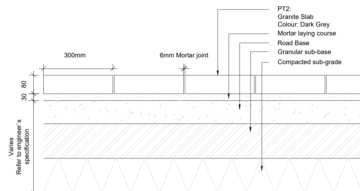
2 PT2: Granite slabs scale 1:10 @A1
