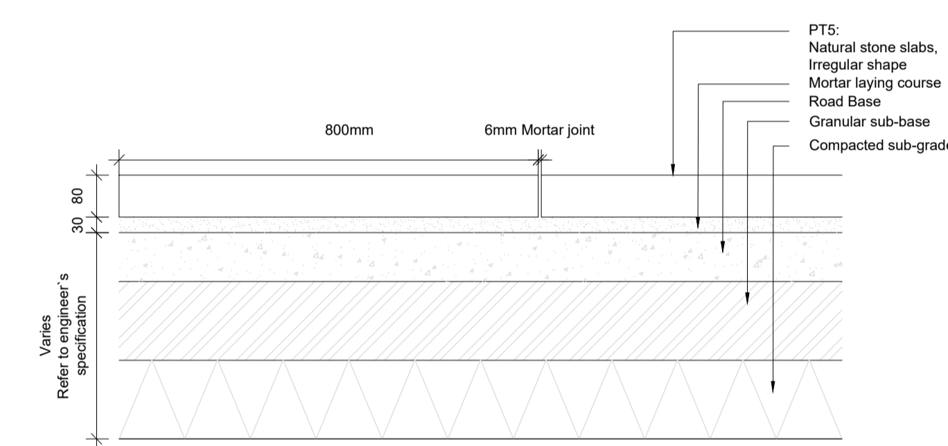
5 PT5: Natural stone slabs, Irregular shape scale 1:10 @A1
